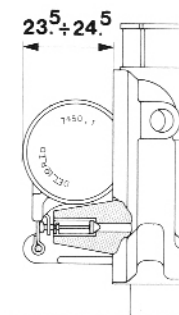
float-pin vertical
